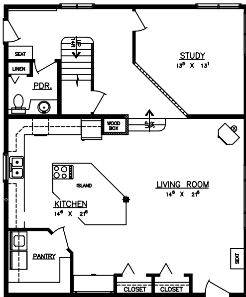
MAIN FLOOR AREA = 1080 S.F.
